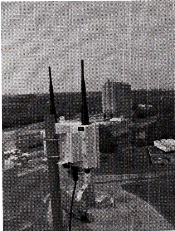
Figure 3 Wave Relay™ installation.
