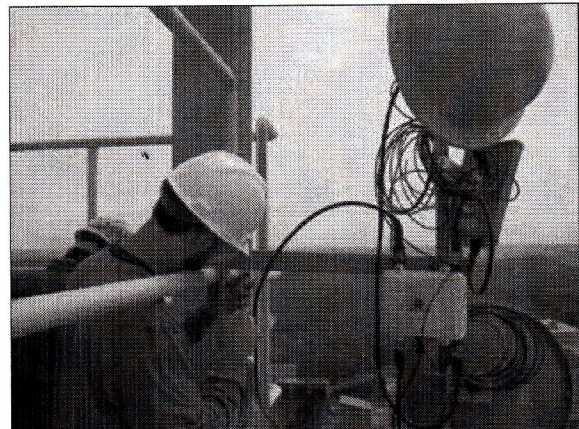
Figure 2 Installation of sector antennas and wireless router.
