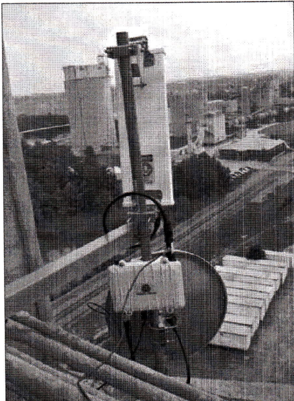
Figure 4 2.4 GHz sector and 5.8 GHz backhaul dish antenna
